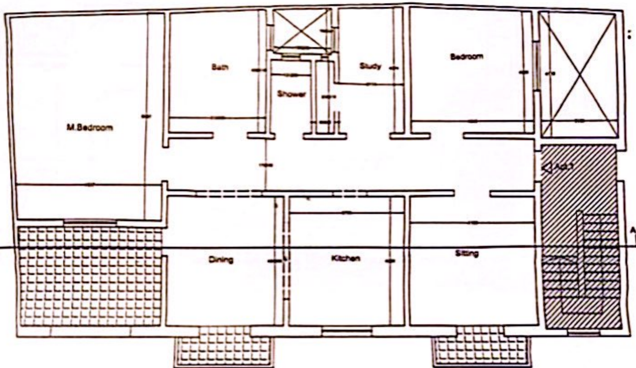
As Built First Floor Scale 1:100
