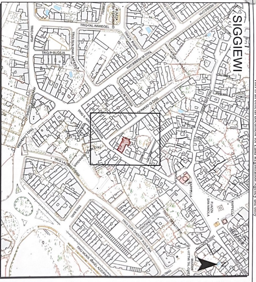
Pjanta tas-Sit 1:2500 Site Plan
